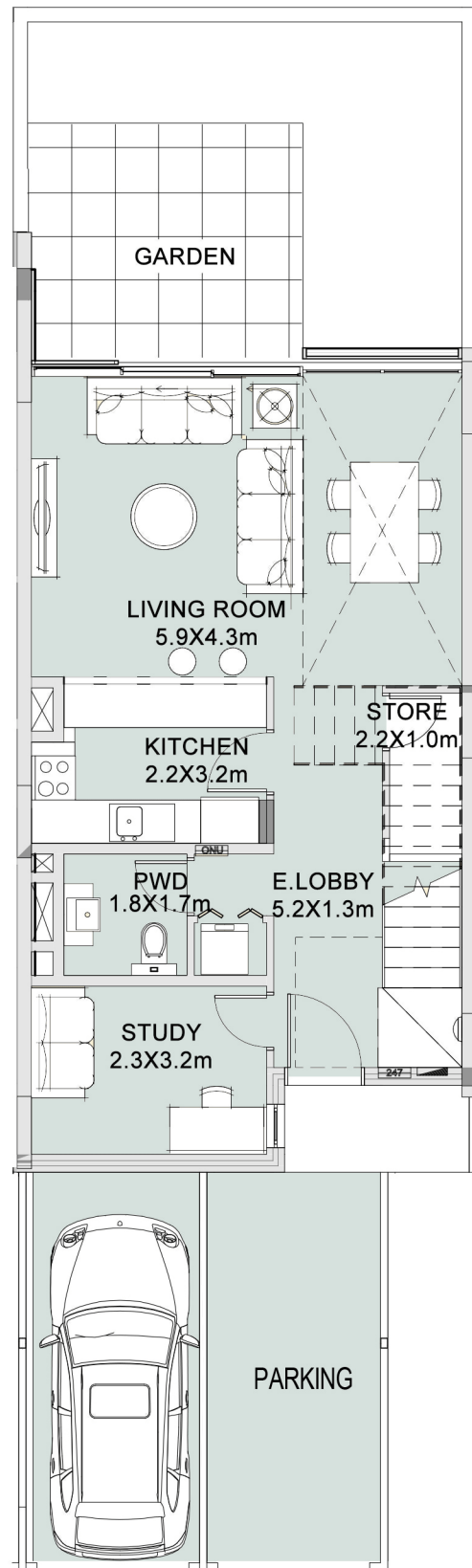
A-2-2B | Ground Level 1:100
