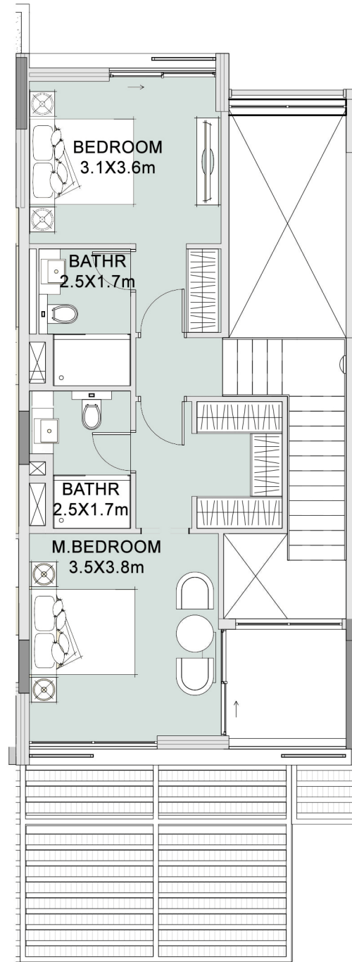
A-2-2B | Level 1 1:100
